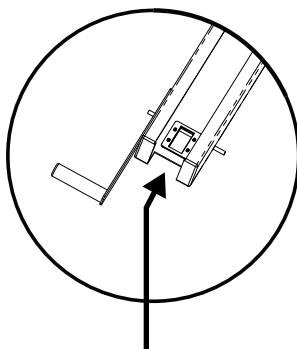
2. Stack two spacer plates in position over bolt holes (on the inside of the rack)
