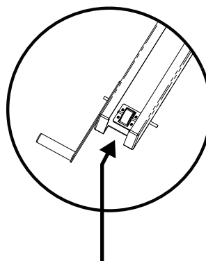
3. Reassemble wheel and axle (axle rests on top face of stacked spacers)
